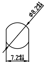
SUGGESTED PANEL CUT OUT
